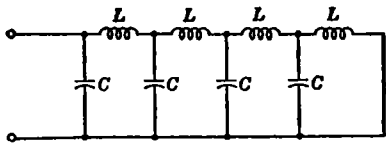
FIG. 6-32.—Current-fed pulse-forming network of the uniform-line type.
